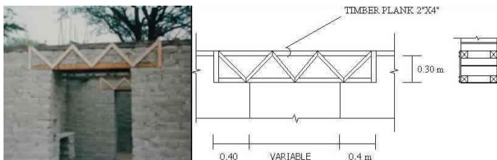
Seismic Strengthening - Cane Reinforcement of Adobe Walls
