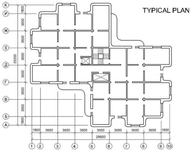
Plan of a Typical Building
